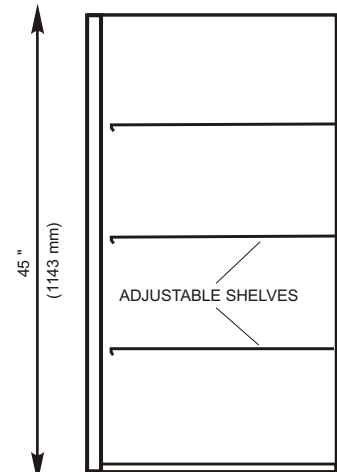
SECTION
